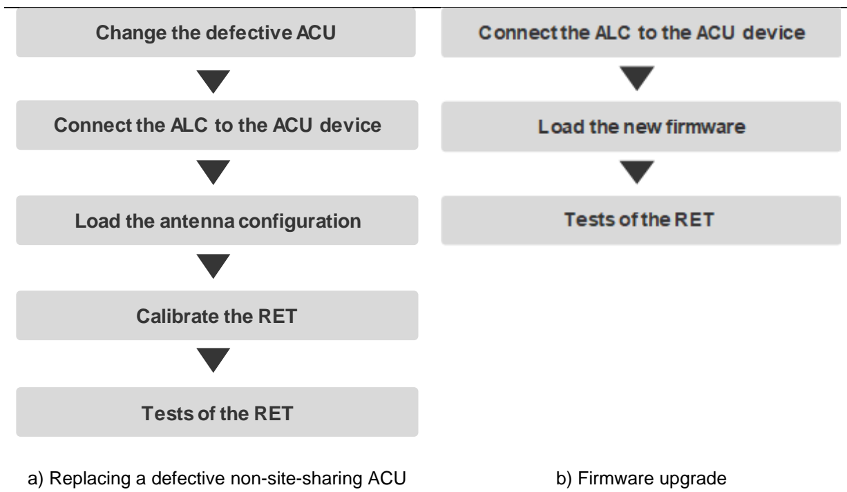
Figure 1: Flowchart for maintaining a non-site-sharing ACU
