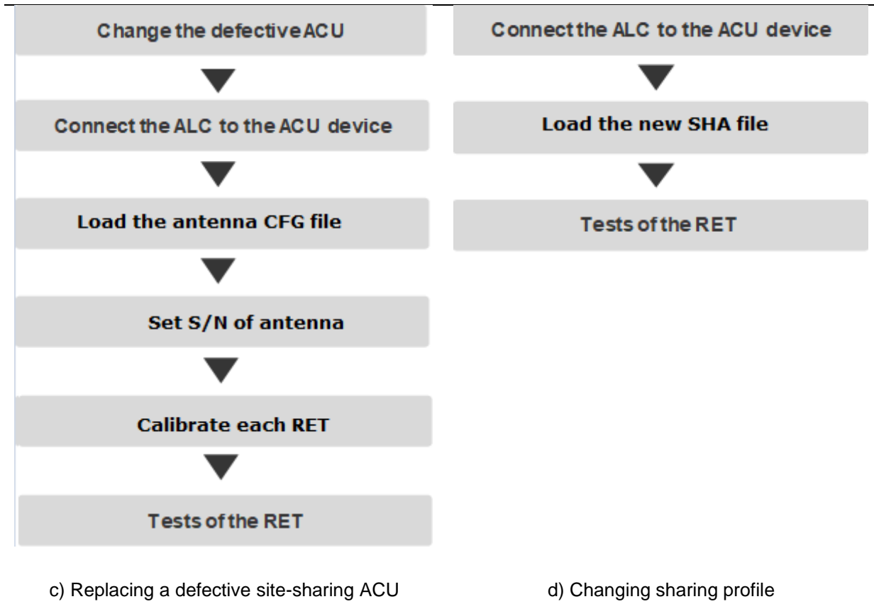
Figure 1: Flowchart for maintaining a site-sharing ACU
